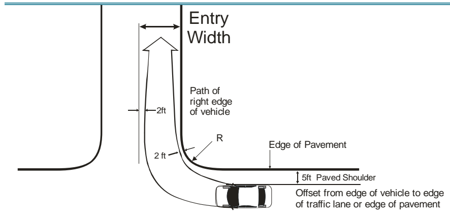
Exhibit 14 MEASURES IMPORTANT TO DETERMINING THE ENTRY OPERATIONS OF A DRIVEWAY
