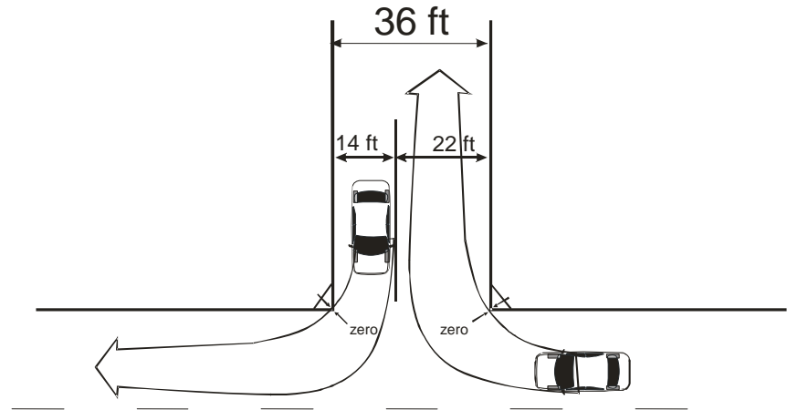
Dropped Curb
