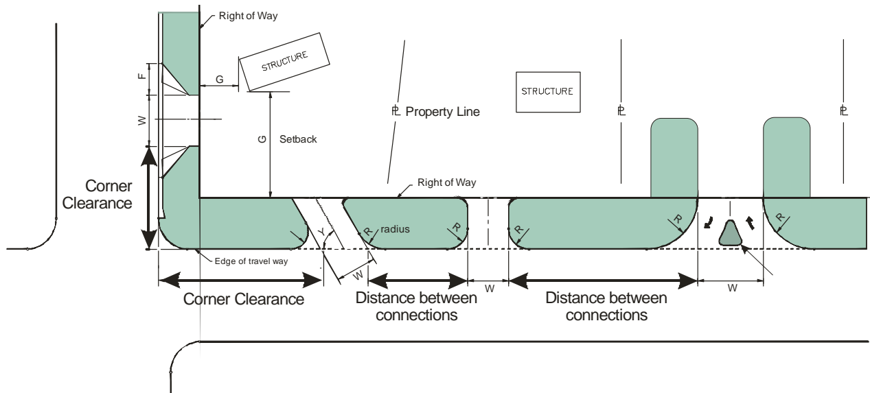
Exhibit 56 DRIVEWAY LOCATION
