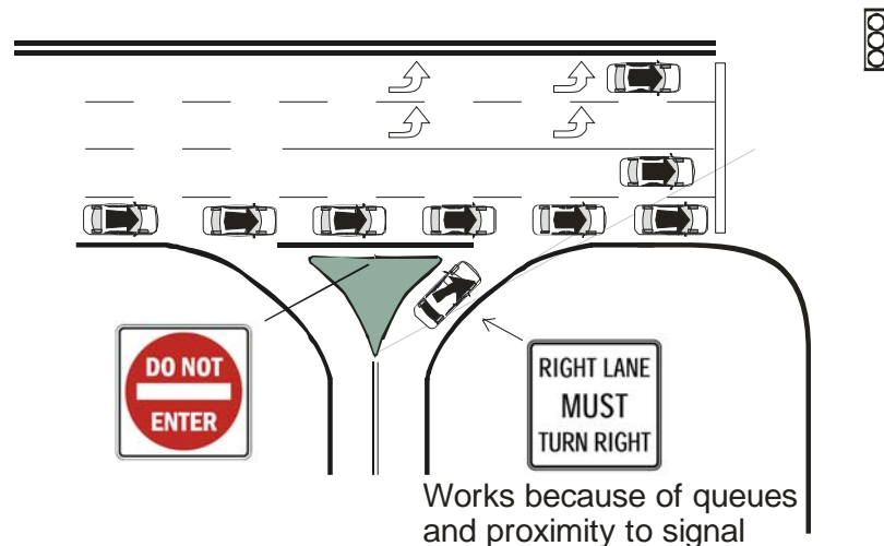
Exhibit 32 “PORK CHOP” CLOSE TO AN INTERSECTION
