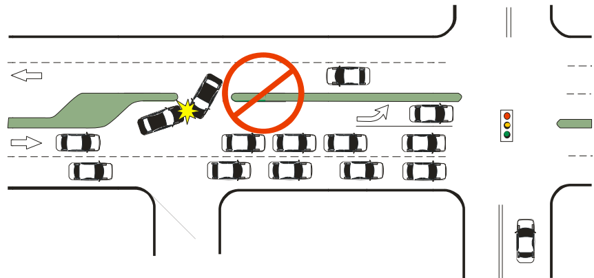
Exhibit 63 NO MEDIAN OPENINGS ACROSS LEFT TURN LANE
