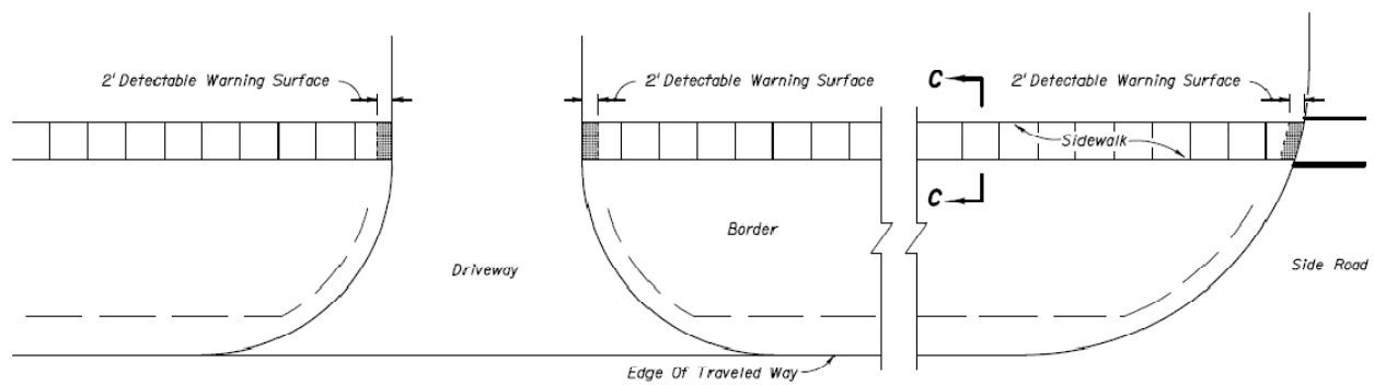
DISCONTINUOUS SIDEWALK PLAN
