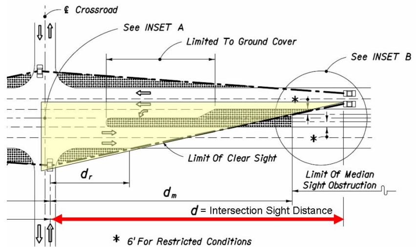
Exhibit 49 Intersection Sight Distance with Clear Sight Triangle
