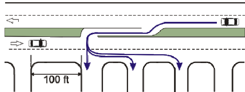
Exhibit 64 ENTRY MANEUVERS FROM A U-TURN
