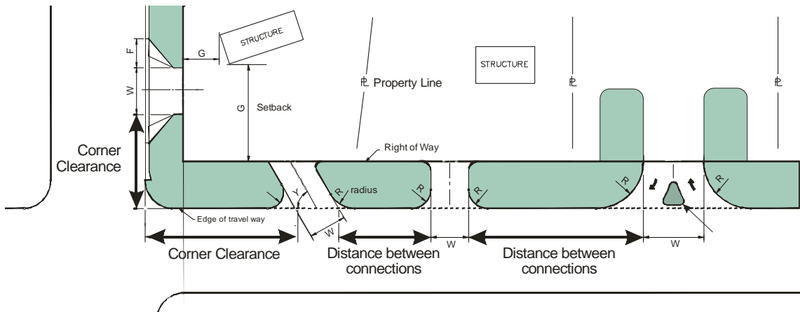
Exhibit 59 DRIVEWAY SEPARATION AND CORNER CLEARANCE
