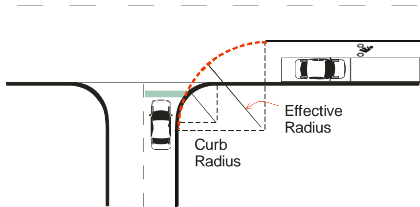
Exhibit 9 Bike lanes can add to the effective radius of the driveway – but use it wisely
