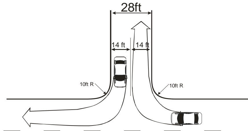
Curb Return Radius
