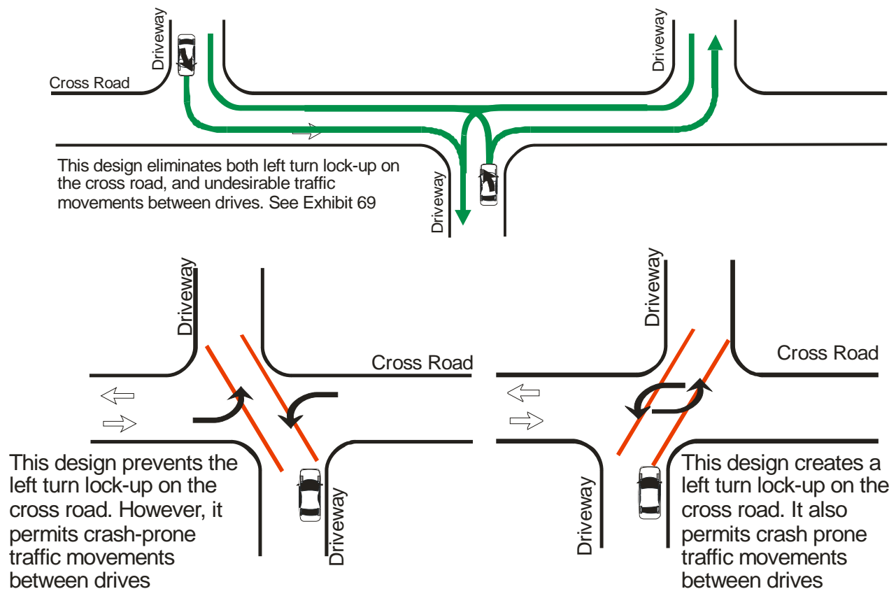
Exhibit 68 AVOID JOG MANEUVERS
