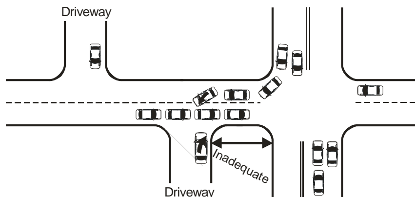
Exhibit 57 CORNER CLEARANCE
